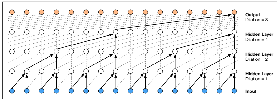
Figure 16.15 Dilated convolutions, showing one dilation cycle size of 4, i.e., dilation values of 1, 2, 4, 8. Figure from van den Oord et al. (2016) .
