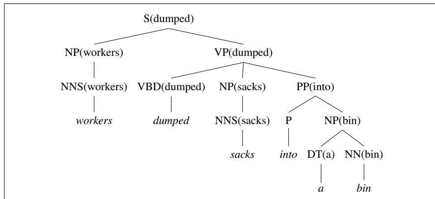
Figure 17.16 A lexicalized tree from Collins (1999).
